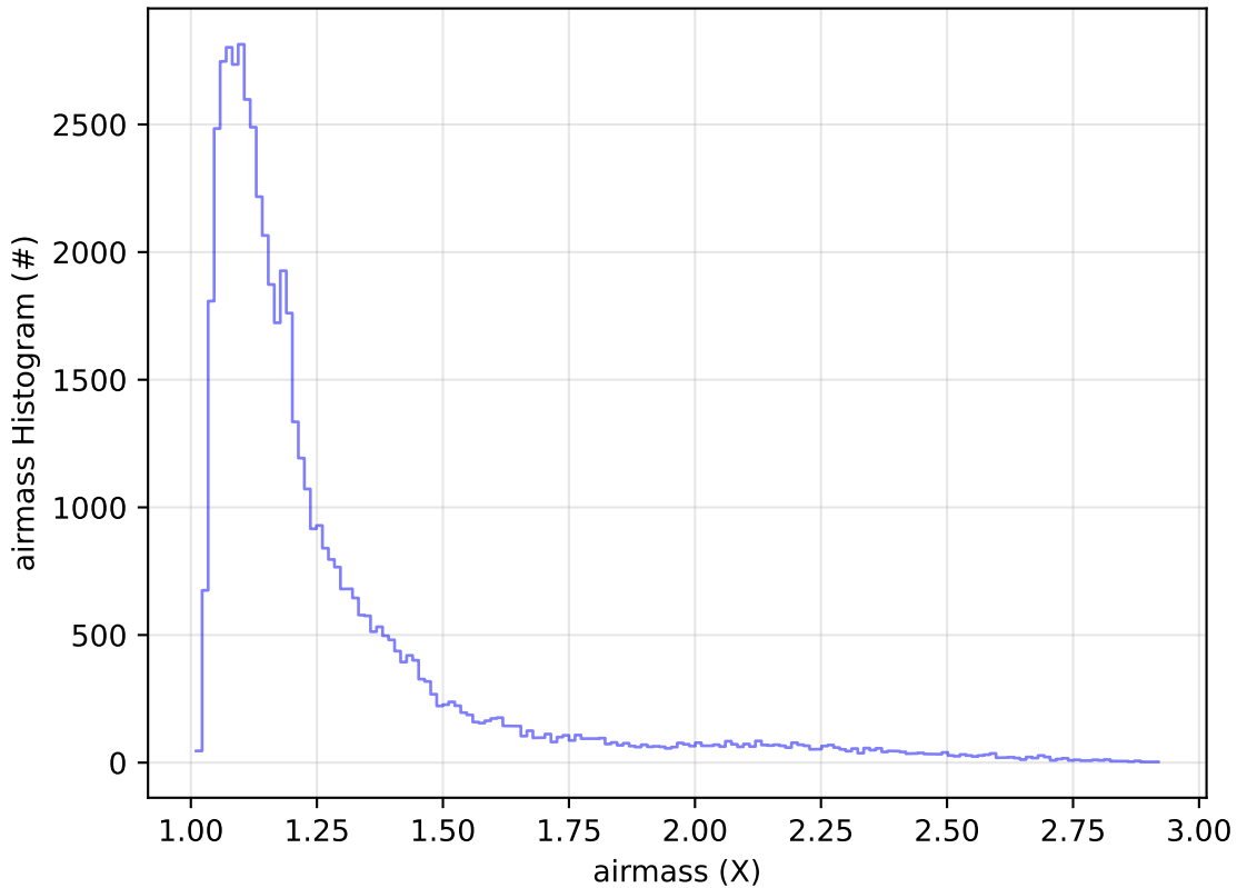
too_elab_2yr_r64_d3_ugrizy_v3.4_10yrs Yr 1 i band: airmass Histogram
