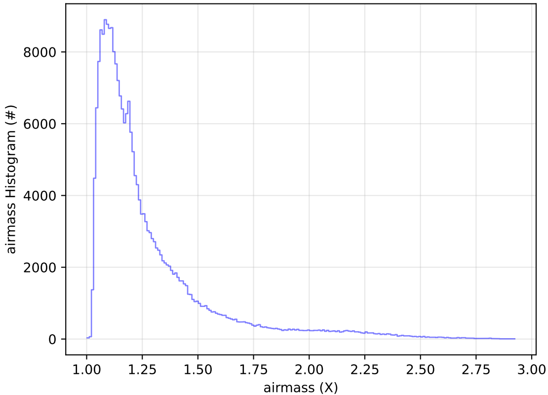
too_elab_2yr_r64_d3_ugrizy_v3.4_10yrs Yr 1 all bands: airmass Histogram
