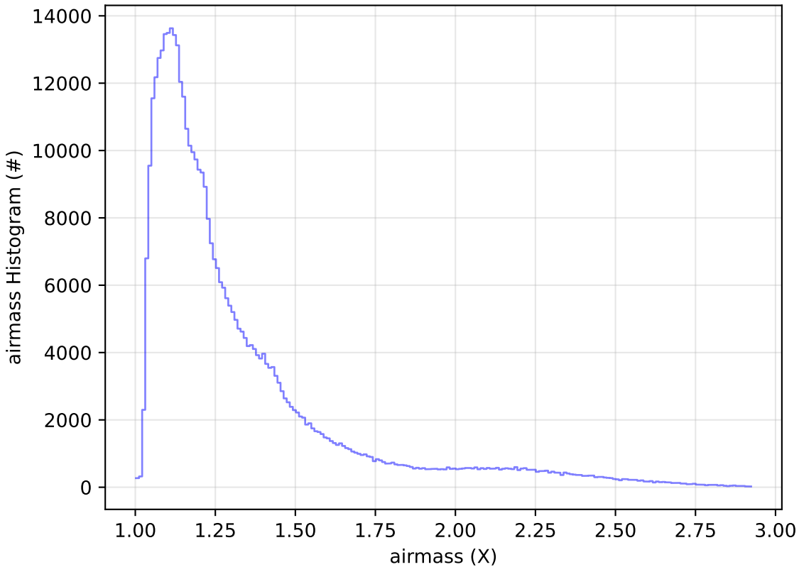
too_elab_2yr_r64_d3_ugrizy_v3.4_10yrs WFD z band: airmass Histogram
