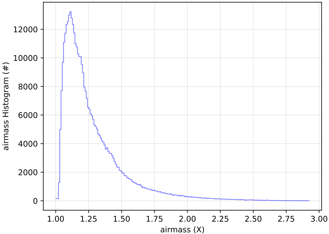
too_elab_2yr_r64_d3_ugrizy_v3.4_10yrs WFD y band: airmass Histogram
