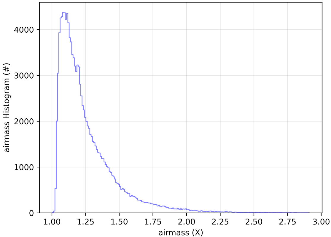
too_elab_2yr_r64_d3_ugrizy_v3.4_10yrs WFD u band: airmass Histogram
