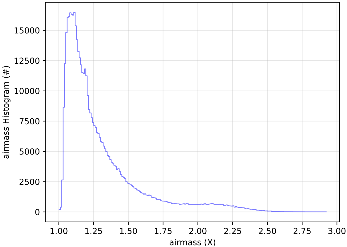
too_elab_2yr_r64_d3_ugrizy_v3.4_10yrs WFD r band: airmass Histogram
