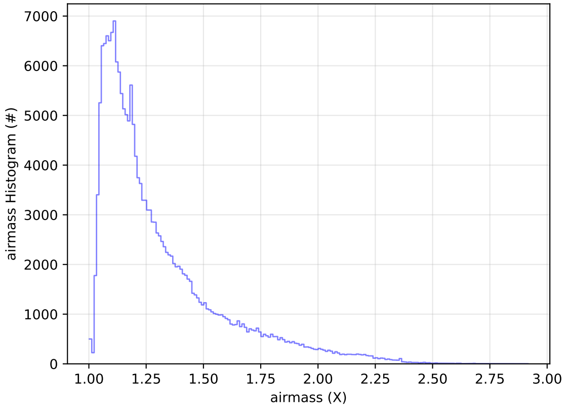
too_elab_2yr_r64_d3_ugrizy_v3.4_10yrs WFD g band: airmass Histogram
