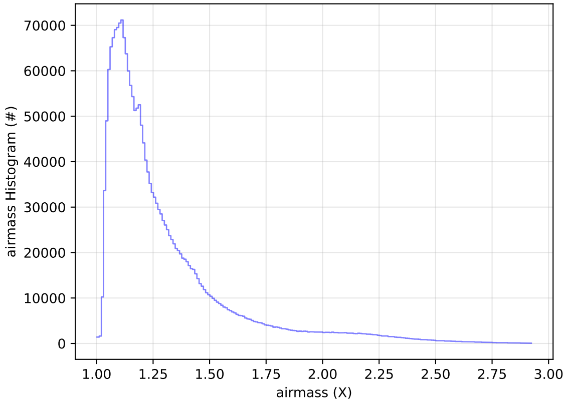
too_elab_2yr_r64_d3_ugrizy_v3.4_10yrs WFD all bands: airmass Histogram
