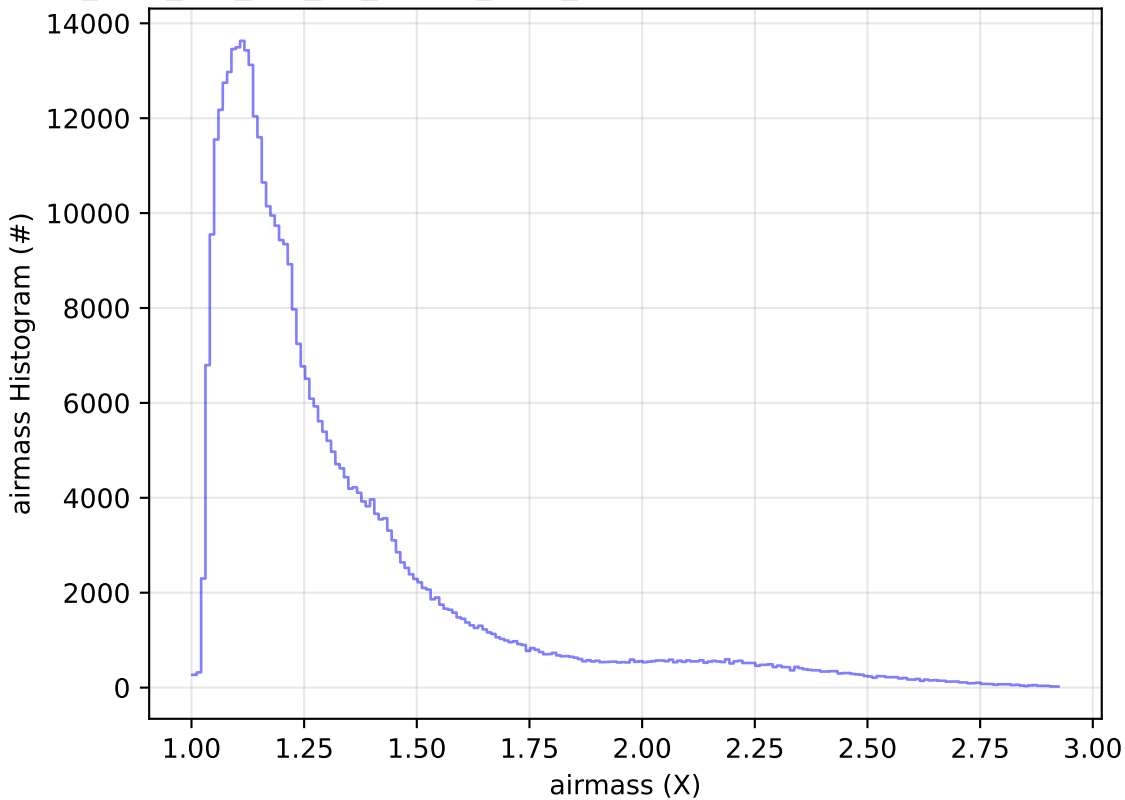
too_elab_2yr_r64_d3_ugrizy_v3.4_10yrs All sky z band: airmass Histogram
