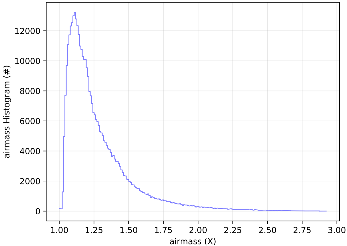
too_elab_2yr_r64_d3_ugrizy_v3.4_10yrs All sky y band: airmass Histogram
