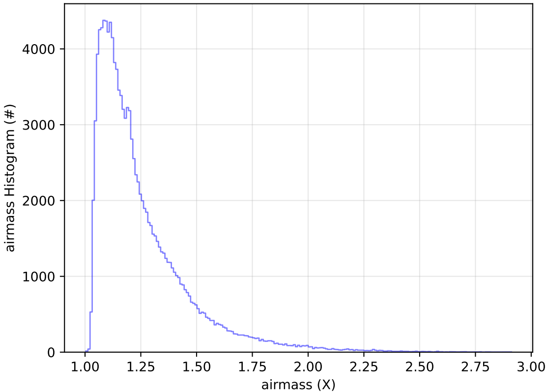
too_elab_2yr_r64_d3_ugrizy_v3.4_10yrs All sky u band: airmass Histogram
