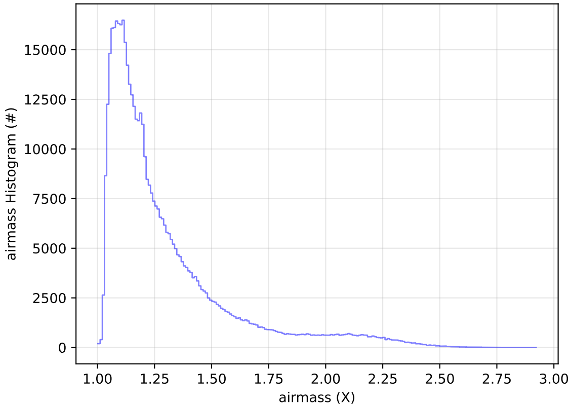
too_elab_2yr_r64_d3_ugrizy_v3.4_10yrs All sky r band: airmass Histogram
