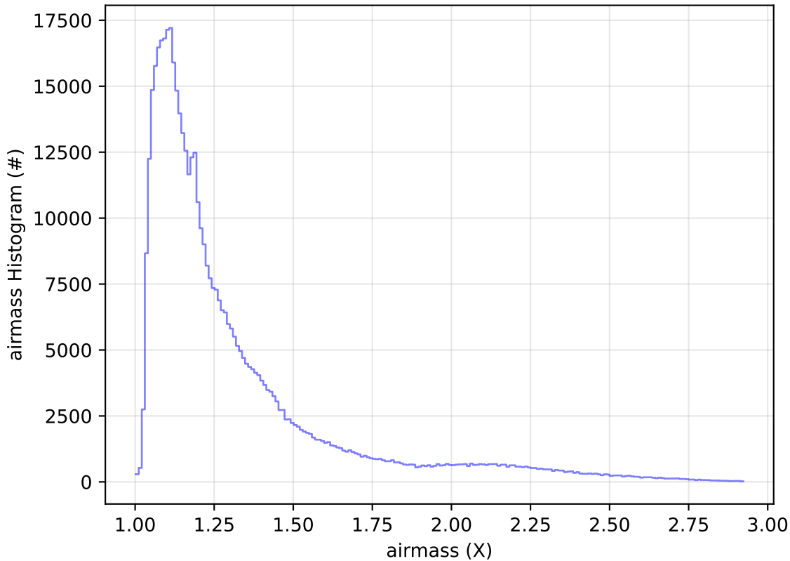
too_elab_2yr_r64_d3_ugrizy_v3.4_10yrs All sky i band: airmass Histogram
