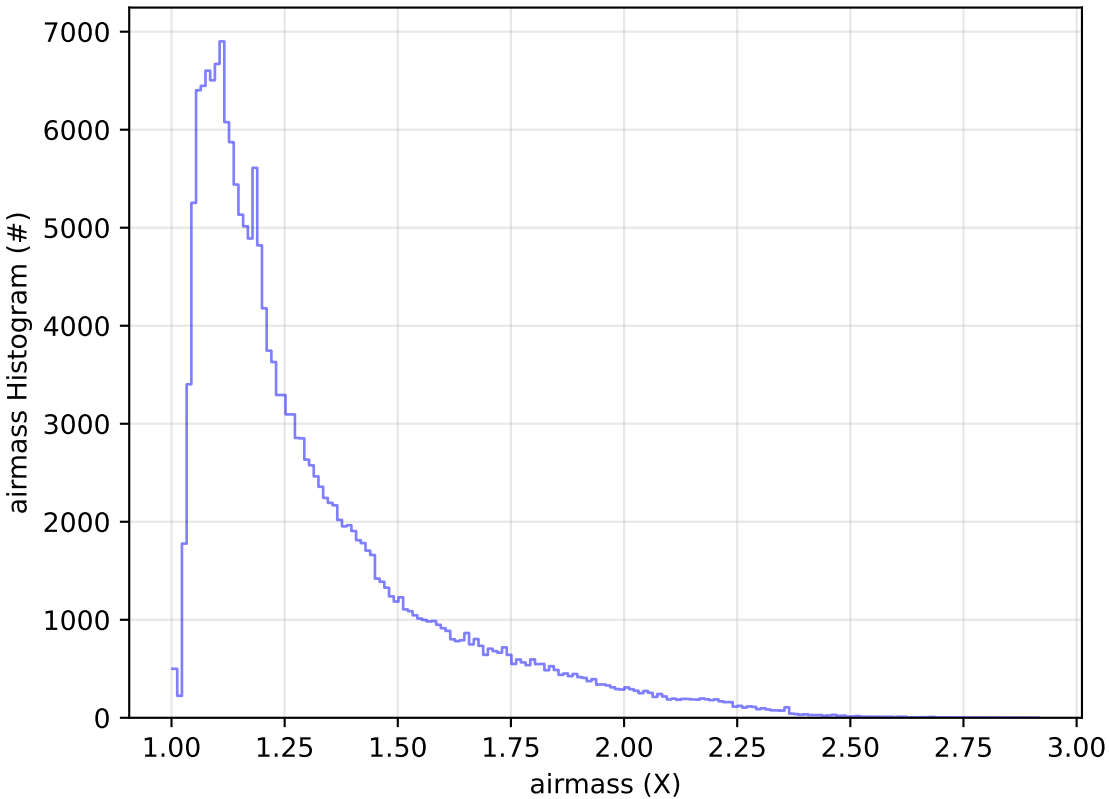
too_elab_2yr_r64_d3_ugrizy_v3.4_10yrs All sky g band: airmass Histogram
