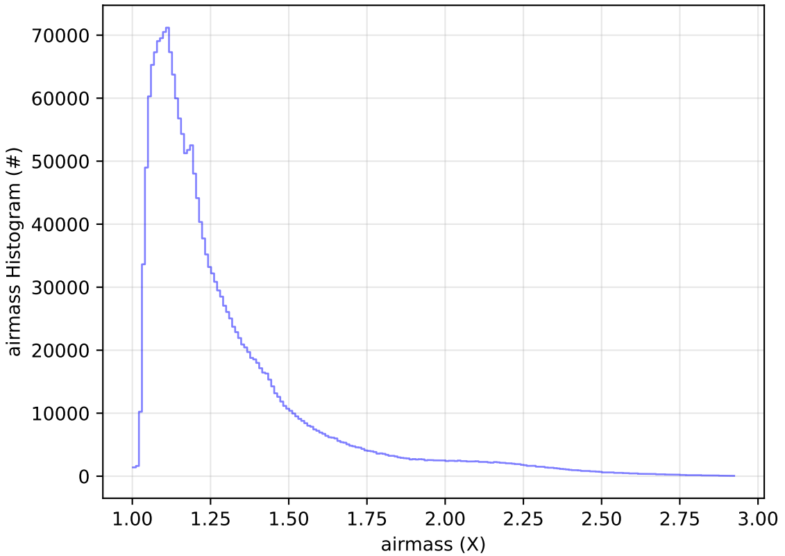
too_elab_2yr_r64_d3_ugrizy_v3.4_10yrs All sky all bands: airmass Histogram
