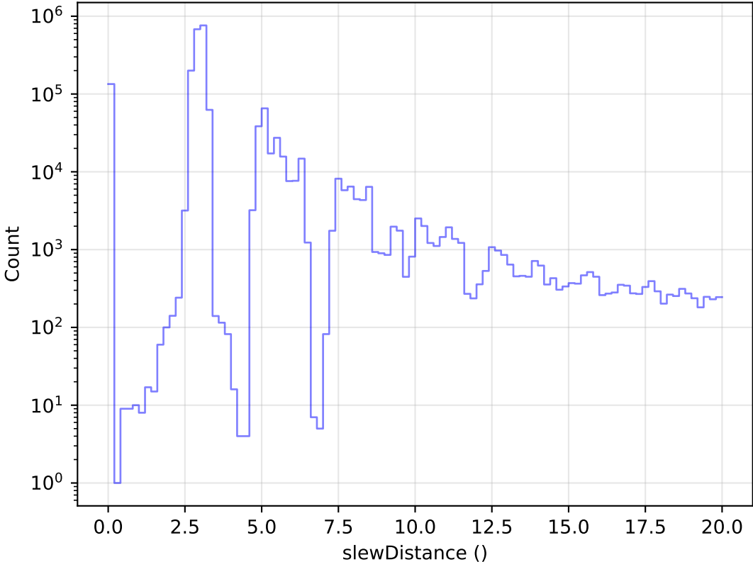
too_elab_2yr_r64_d3_ugrizy_v3.4_10yrs All visits: Zoom Slew Distance Histogram
