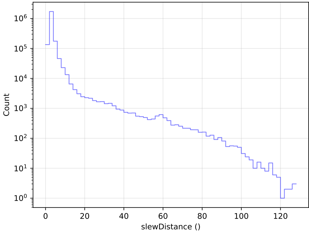
too_elab_2yr_r64_d3_ugrizy_v3.4_10yrs All visits: Slew Distance Histogram
