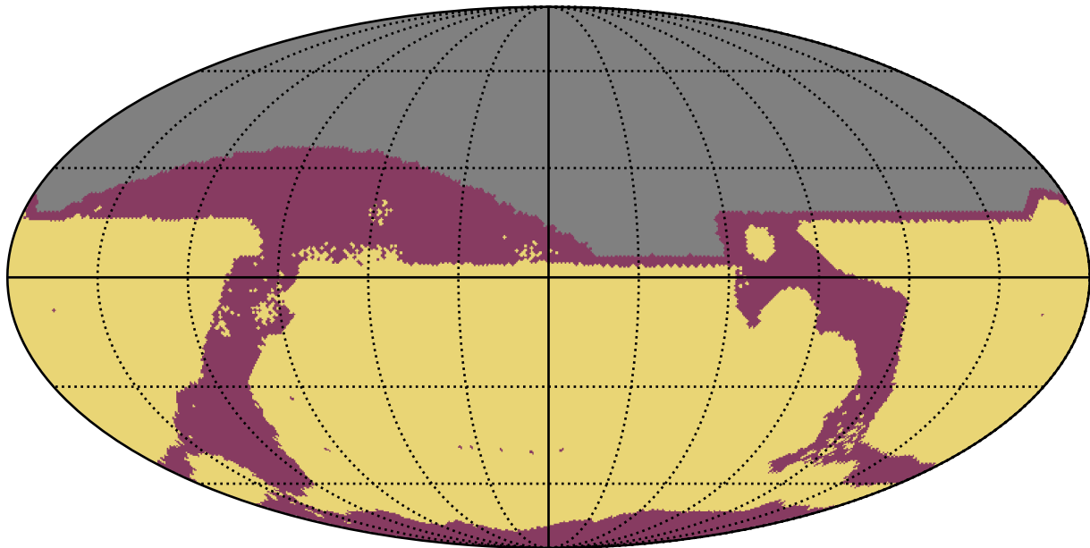
too_elab_2yr_r64_d3_ugrizy_v3.4_10yrs All sky: RapidRevisits
