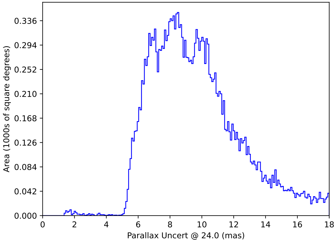
too_elab_2yr_r64_d3_ugrizyv3.4_10yrs All sky: Parallax Uncert @ 24.0
