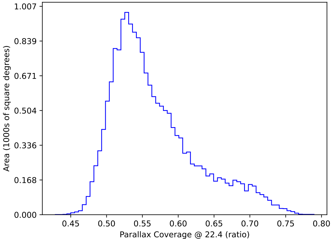
too_elab_2yr_r64_d3_ugrizy_v3.4_10yrs WFD: Parallax Coverage @ 22.4
