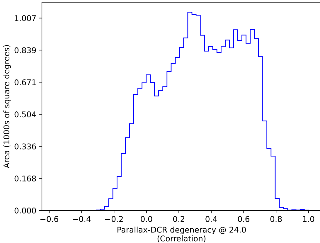
too_elab_2yr_r64_d3_ugrizy_v3.4_10yrs All sky: Parallax-DCR degeneracy @ 24.0
