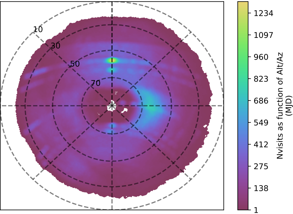
too_elab_2yr_r64_d3_ugrizy_v3.4_10yrs g band: Nvisits as function of Alt/Az
