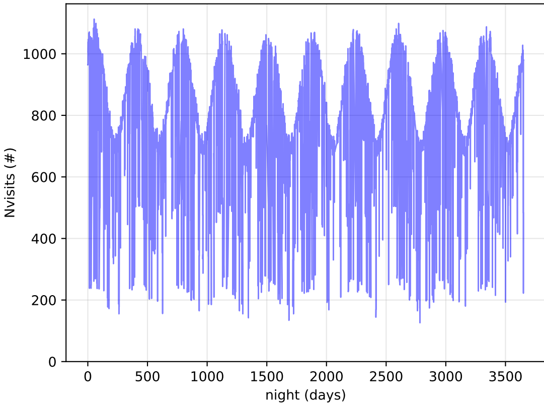
too_elab_2yr_r64_d3_ugrizy_v3.4_10yrs All visits: Nvisits
