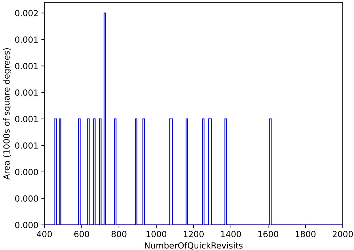
too_elab_2yr_r64_d3_ugrizy_v3.4_10yrs All sky: NumberOfQuickRevisits
