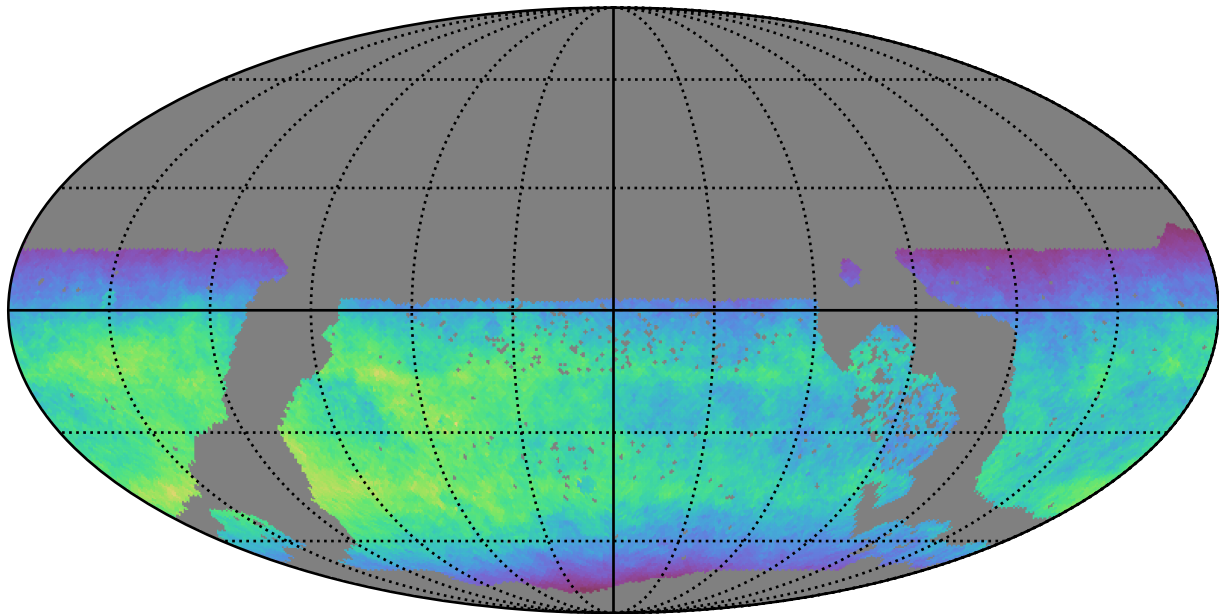
too_elab_2yr_r64_d3_ugrizy_v3.4_10yrs WFD y band: Normalized Teff
