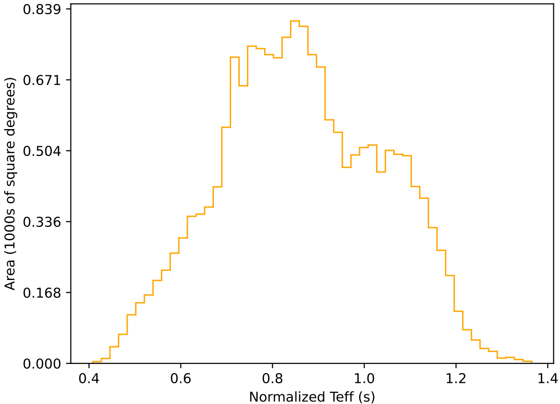
too_elab_2yr_r64_d3_ugrizy_v3.4_10yrs WFD r band: Normalized Teff
