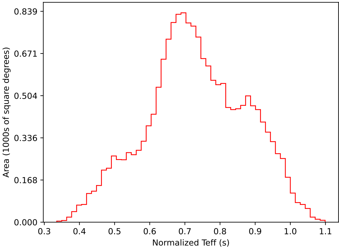
too_elab_2yr_r64_d3_ugrizy_v3.4_10yrs WFD i band: Normalized Teff
