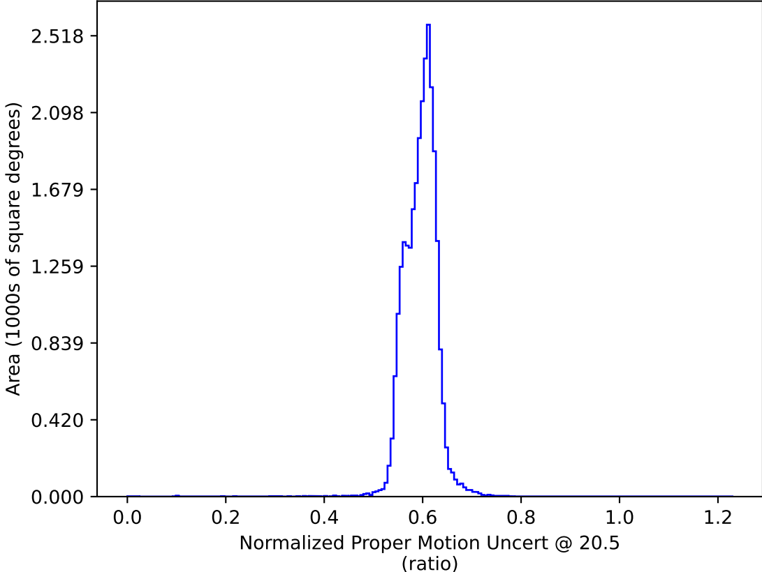
too_elab_2yr_r64_d3_ugrizy_v3.4_10yrs All sky: Normalized Proper Motion Uncert @ 20.5
