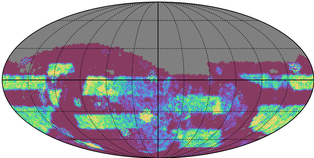
too_elab_2yr_r64_d3_ugrizy_v3.4_10yrs Yr 3-4 z band: NVisits
