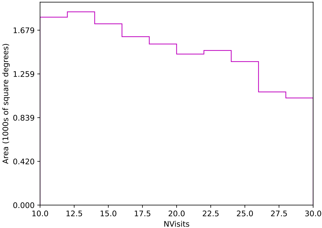
too_elab_2yr_r64_d3_ugrizy_v3.4_10yrs Yr 3-4 z band: NVisits
