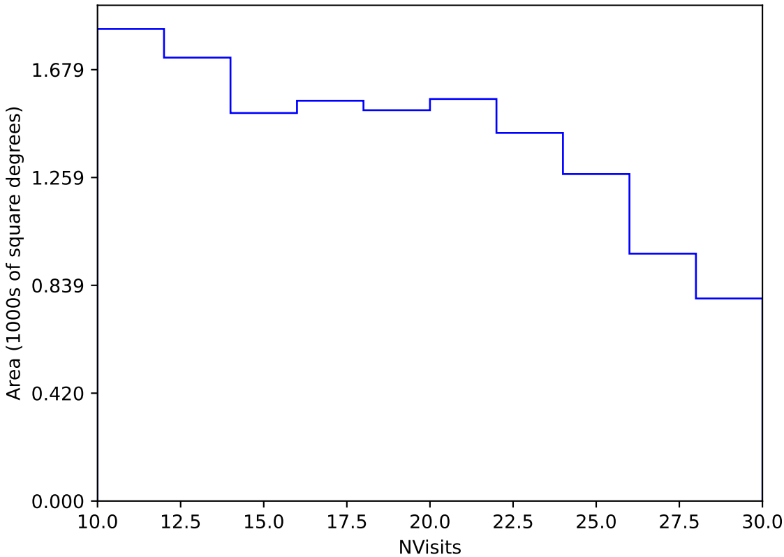
too_elab_2yr_r64_d3_ugrizy_v3.4_10yrs Yr 3-4 y band: NVisits
