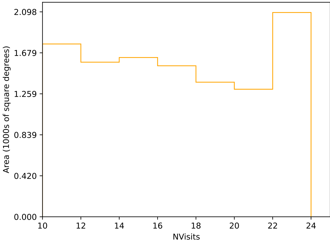
too_elab_2yr_r64_d3_ugrizy_v3.4_10yrs Yr 3-4 r band: NVisits
