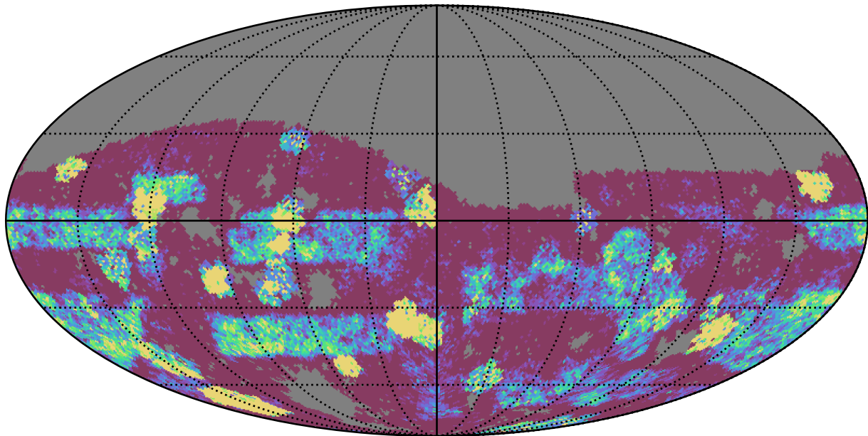
too_elab_2yr_r64_d3_ugrizy_v3.4_10yrs Yr 3-4 g band: NVisits
