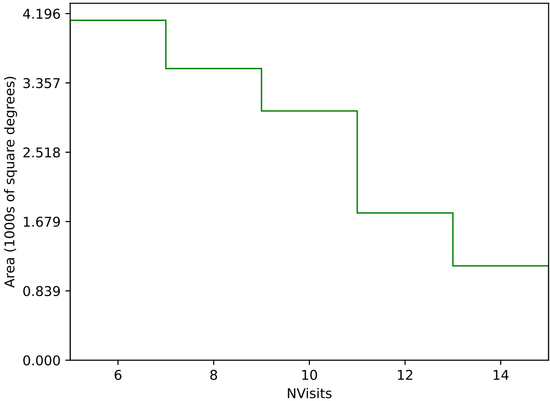
too_elab_2yr_r64_d3_ugrizy_v3.4_10yrs Yr 3-4 g band: NVisits
