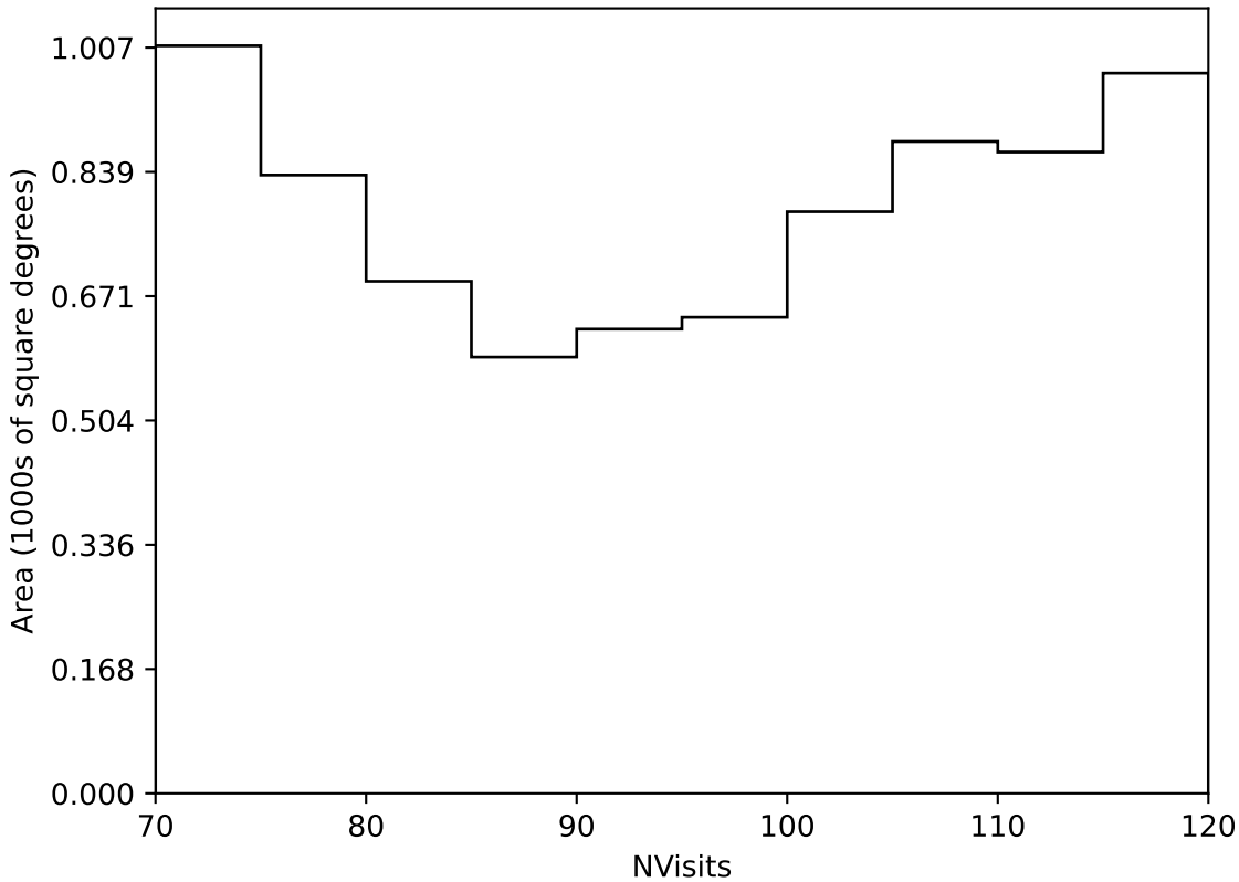
too_elab_2yr_r64_d3_ugrizy_v3.4_10yrs Yr 3-4 all bands: NVisits
