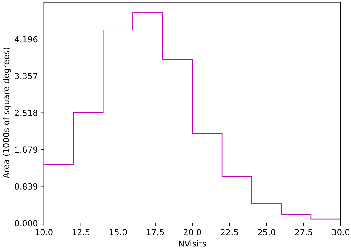
too_elab_2yr_r64_d3_ugrizy_v3.4_10yrs Yr 1 z band: NVisits
