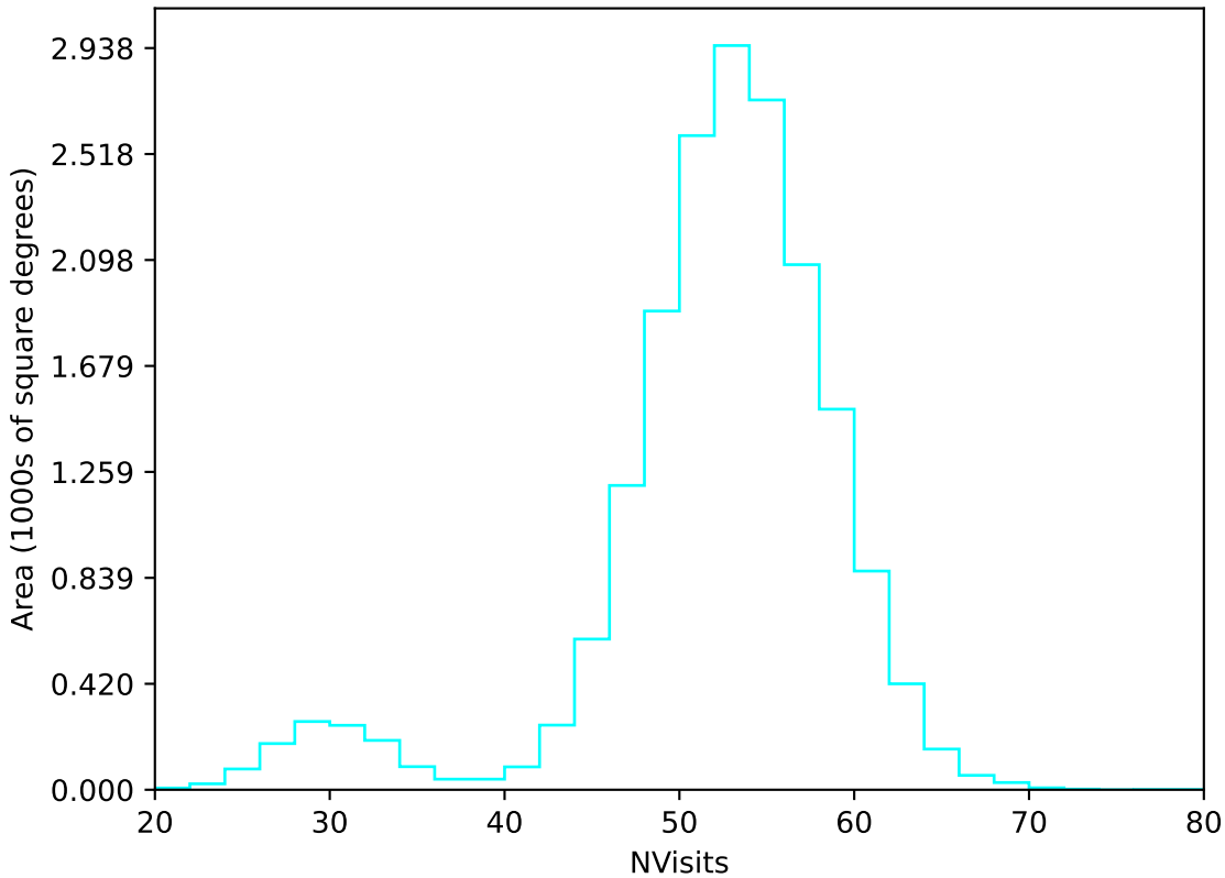
too_elab_2yr_r64_d3_ugrizy_v3.4_10yrs WFD u band: NVisits
