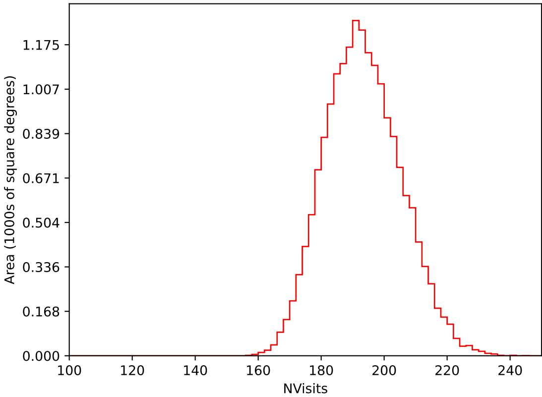
too_elab_2yr_r64_d3_ugrizy_v3.4_10yrs WFD i band: NVisits
