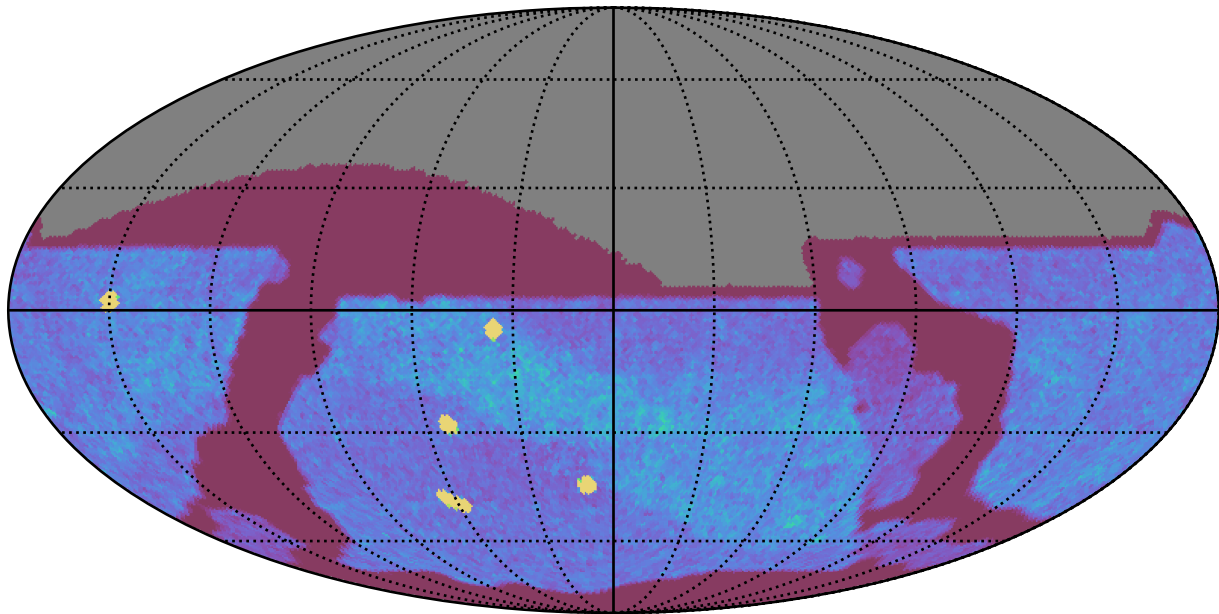
too_elab_2yr_r64_d3_ugrizy_v3.4_10yrs All sky z band: NVisits
