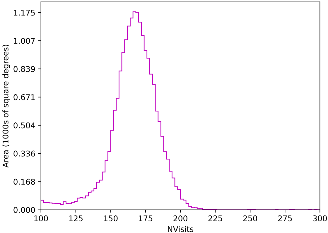
too_elab_2yr_r64_d3_ugrizy_v3.4_10yrs All sky z band: NVisits
