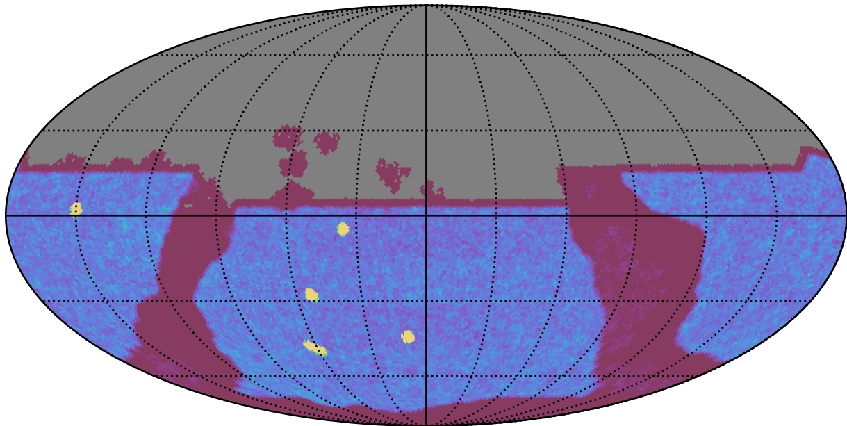
too_elab_2yr_r64_d3_ugrizy_v3.4_10yrs All sky y band: NVisits
