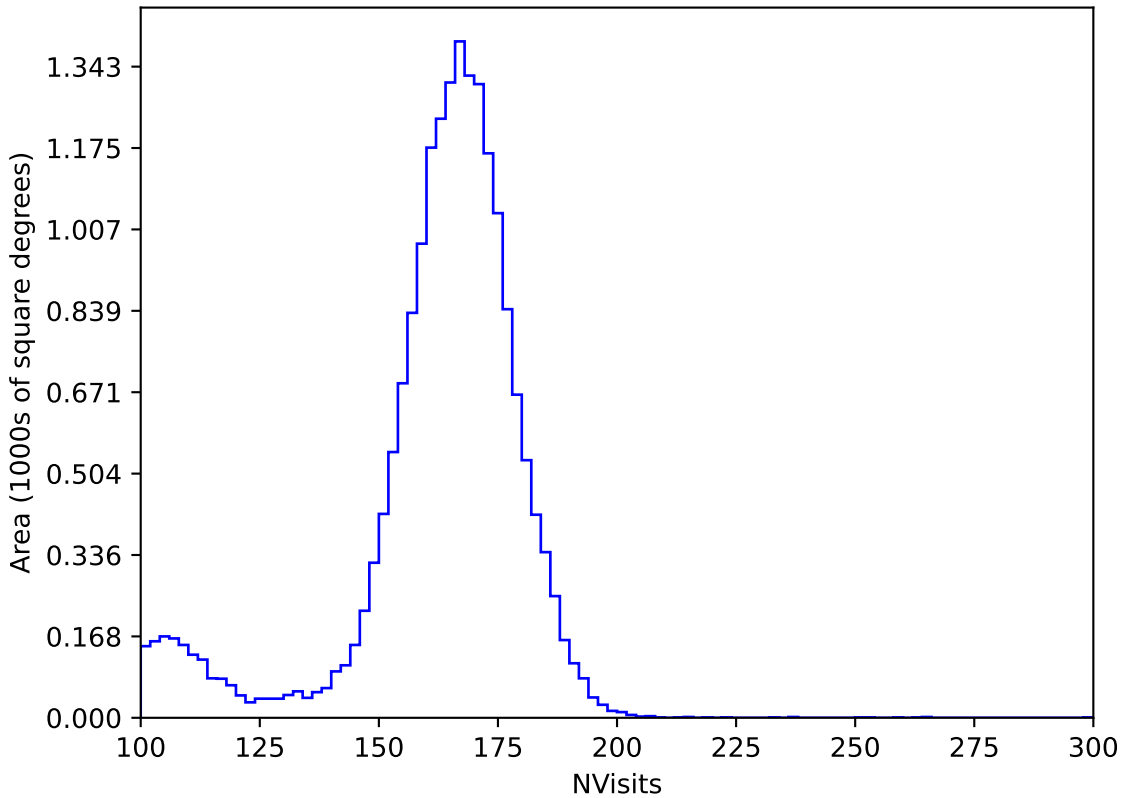
too_elab_2yr_r64_d3_ugrizy_v3.4_10yrs All sky y band: NVisits
