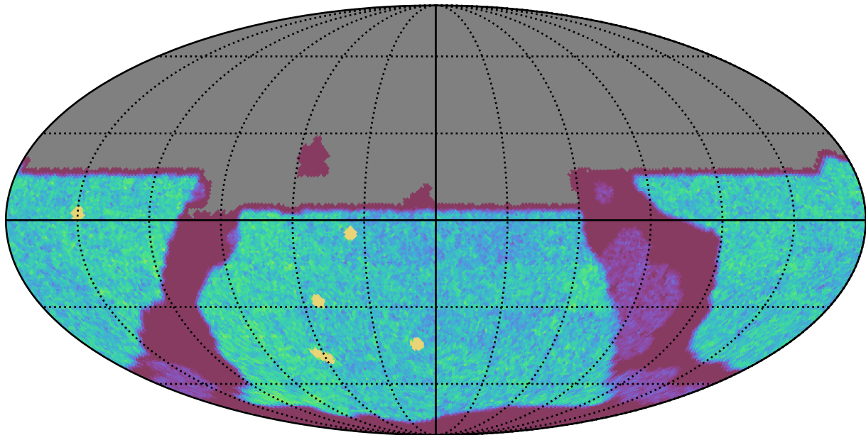
too_elab_2yr_r64_d3_ugrizy_v3.4_10yrs All sky u band: NVisits
