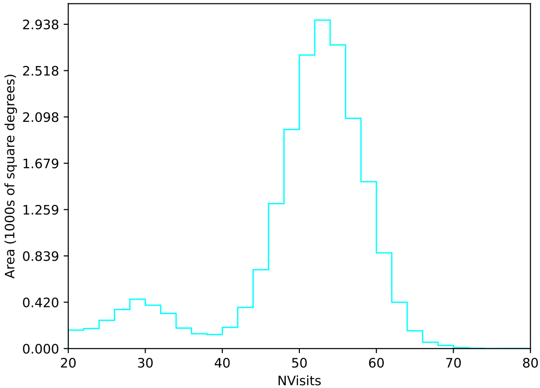
too_elab_2yr_r64_d3_ugrizy_v3.4_10yrs All sky u band: NVisits
