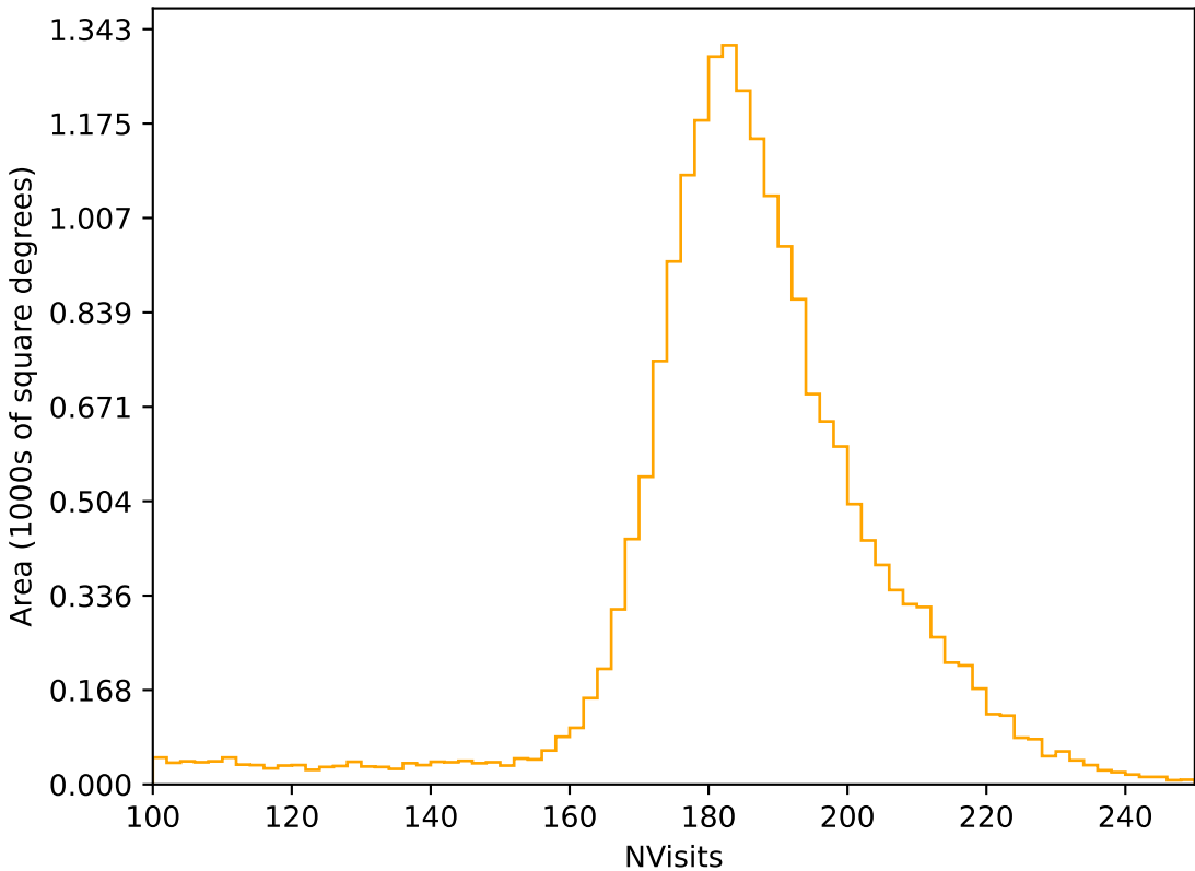
too_elab_2yr_r64_d3_ugrizy_v3.4_10yrs All sky r band: NVisits
