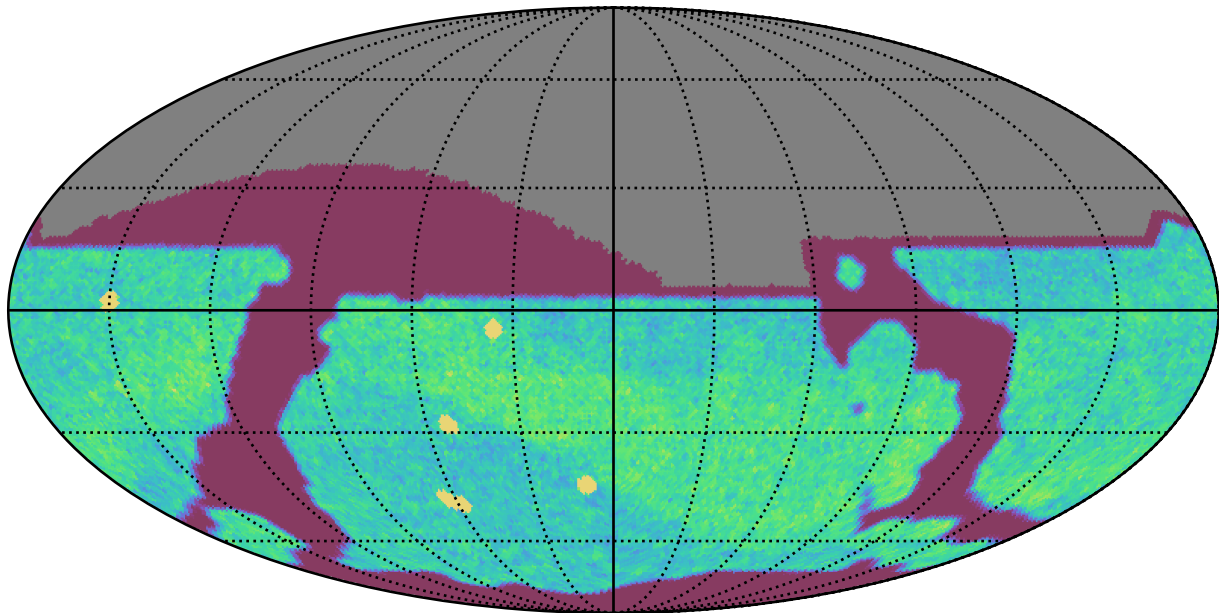
too_elab_2yr_r64_d3_ugrizy_v3.4_10yrs All sky i band: NVisits
