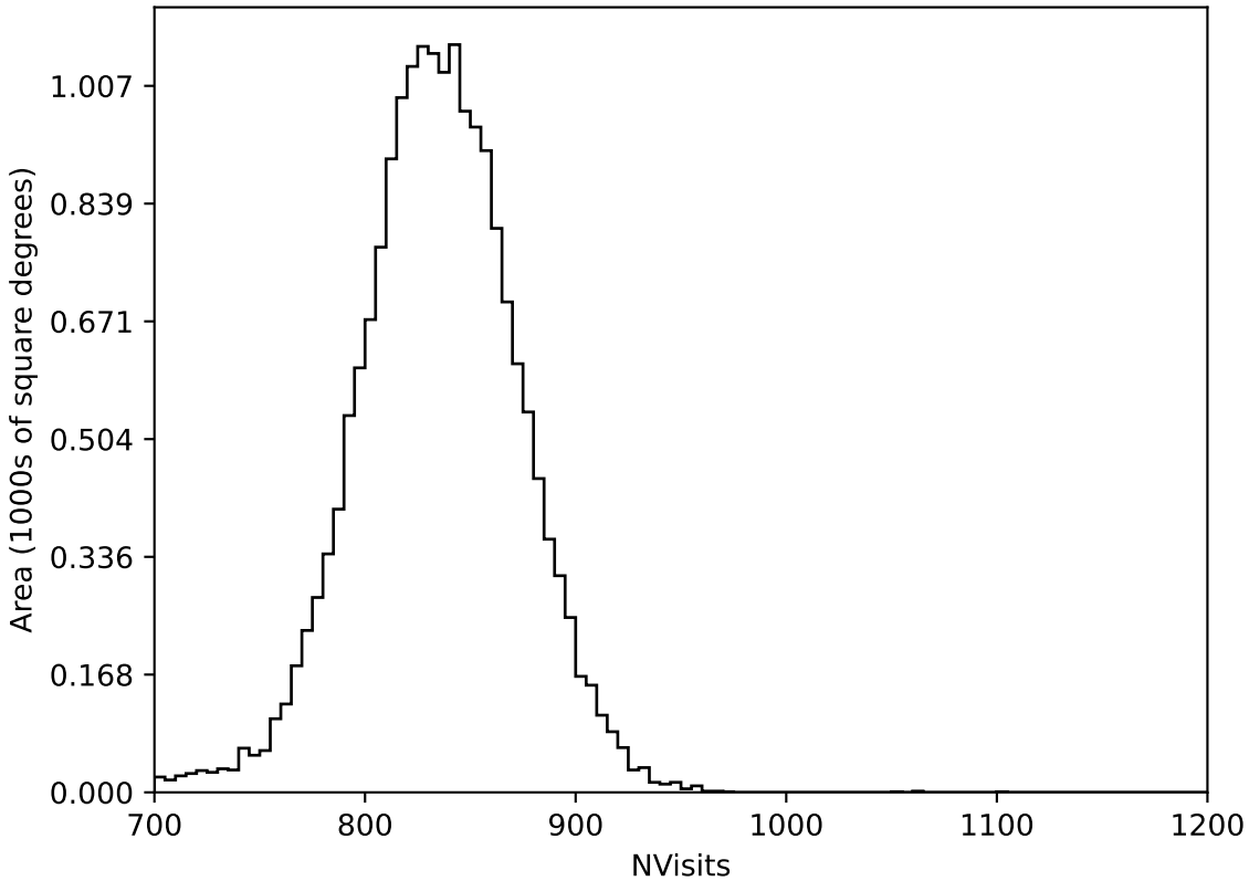
too_elab_2yr_r64_d3_ugrizy_v3.4_10yrs All sky all bands: NVisits
