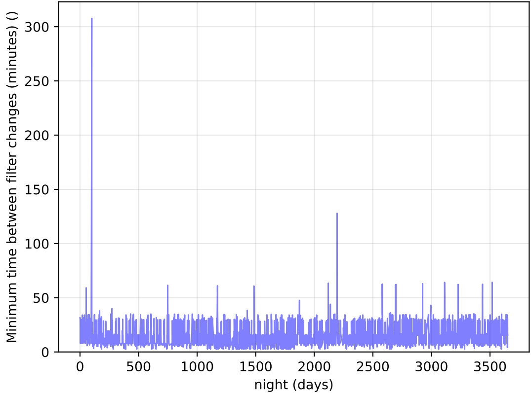
too_elab_2yr_r64_d3_ugrizy_v3.4_10yrs Per Night: Minimum time between filter changes (minutes)
