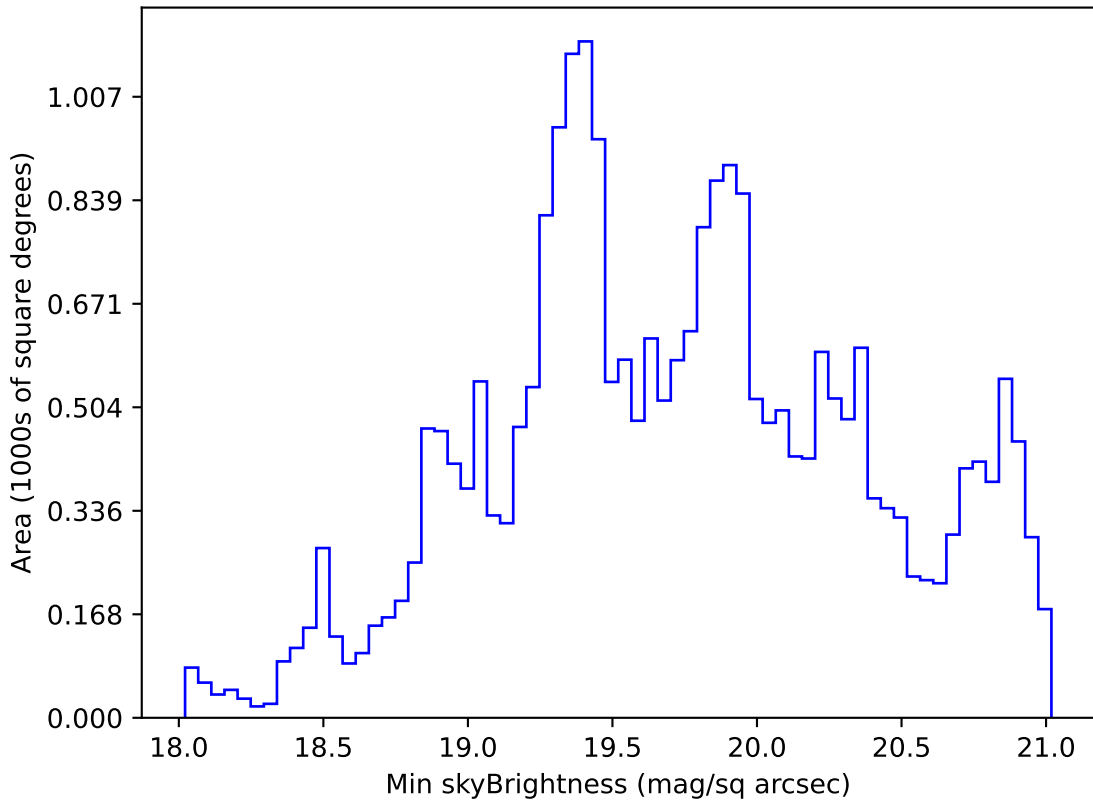
too_elab_2yr_r64_d3_ugrizy_v3.4_10yrs Yr 1 r band: Min skyBrightness
