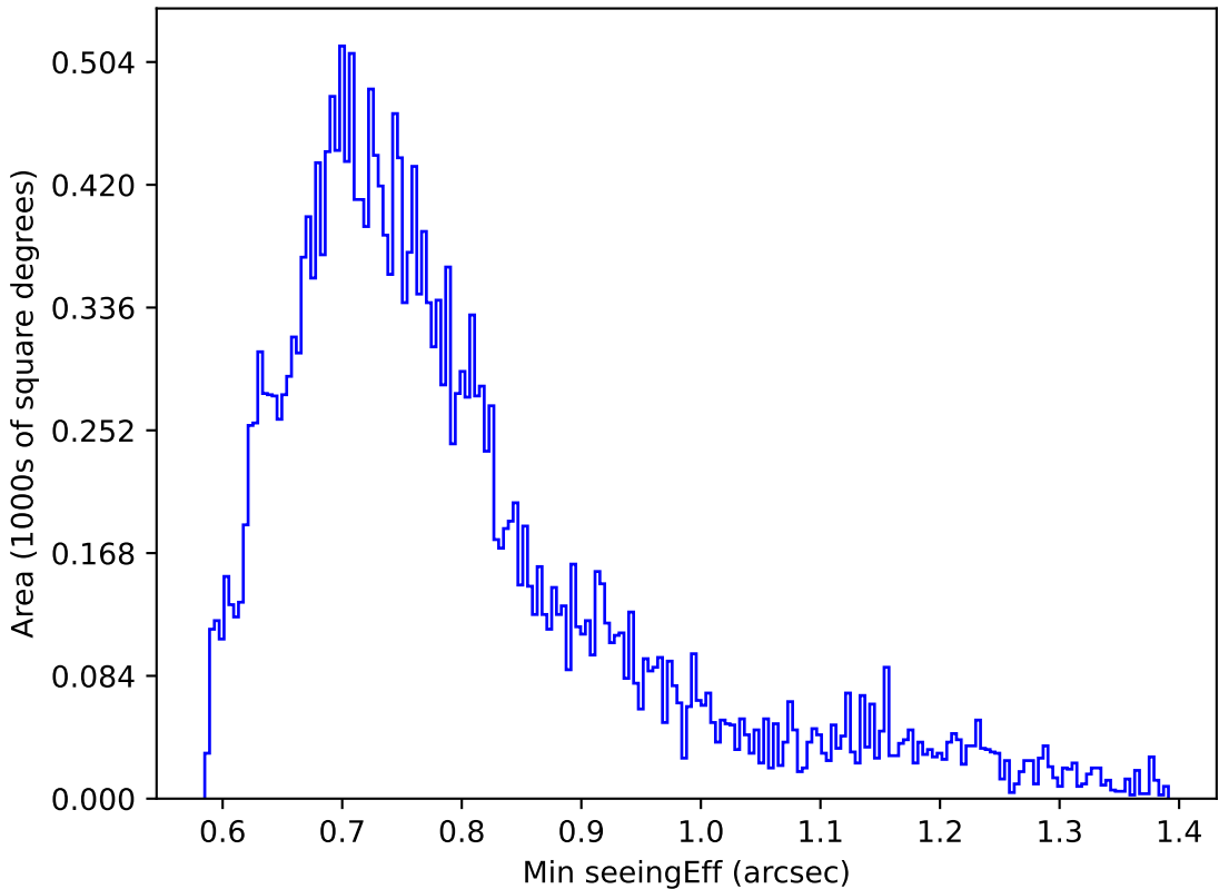
too_elab_2yr_r64_d3_ugrizy_v3.4_10yrs Yr 1 g band: Min seeingEff
